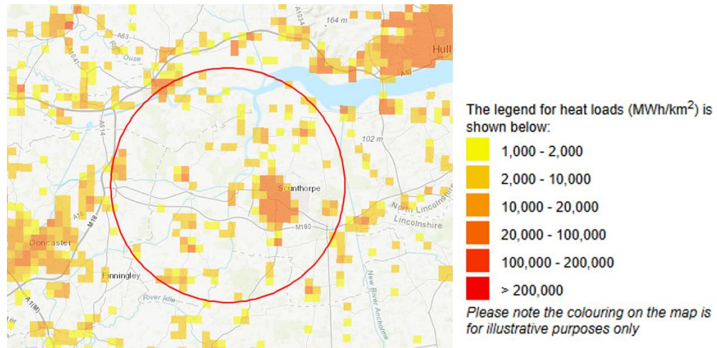
Plate 6: (Appendix B) Results from the examination of the UK CHP Development Map: Total heat demand map
